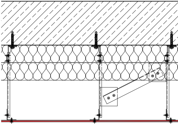
Adjustment range
