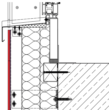
Window sill
