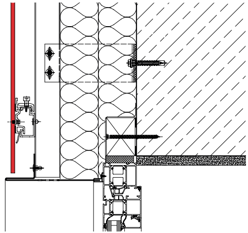
Lintel with metal
