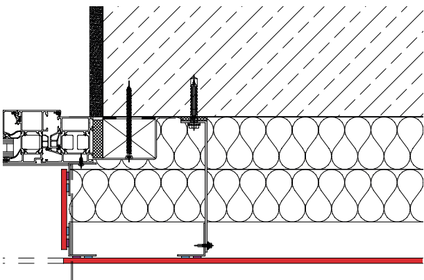
Window reveal with board material
