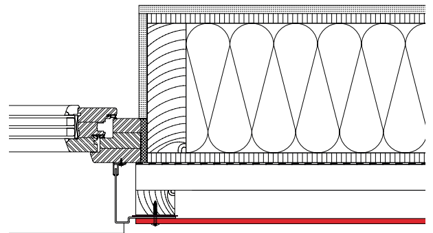
Window reveal with metal
