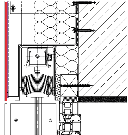
Lintel with Roman blinds
