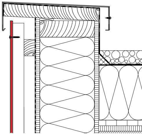
Attic connection
