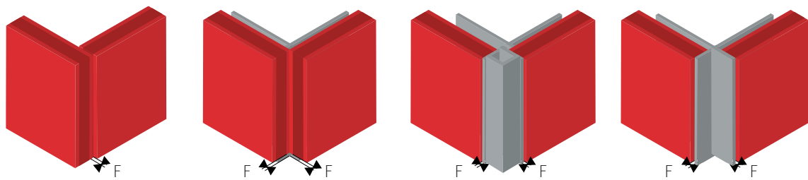
Joint width F = 5 - 10 mm
