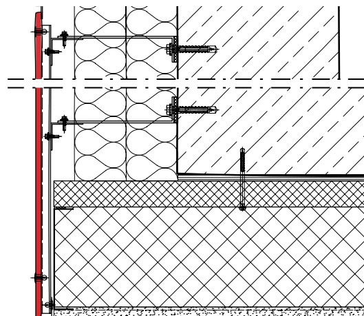
External Corner
