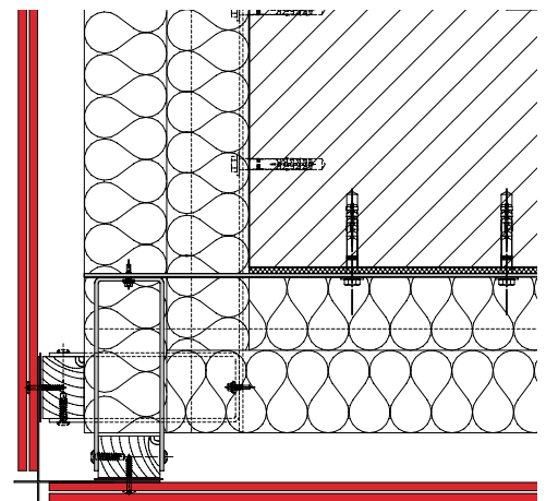
External corner with external corner
