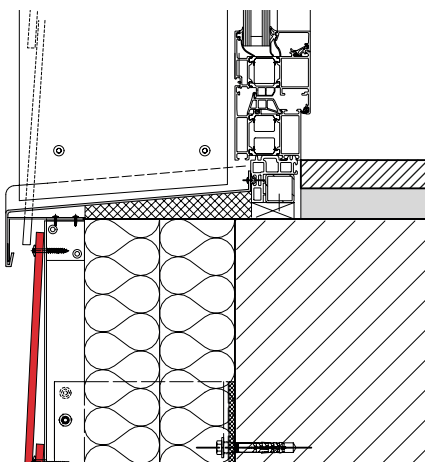
Window sill
