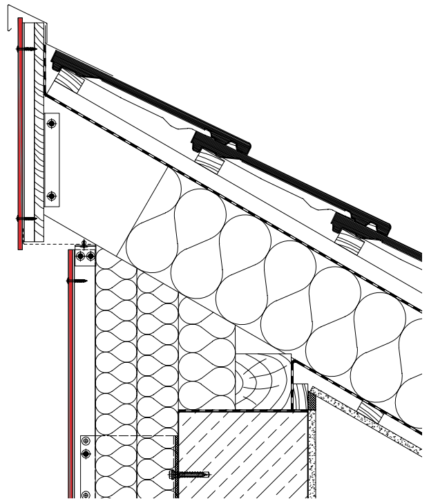
Roof ridge
