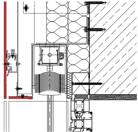
Lintel with Roman blinds
